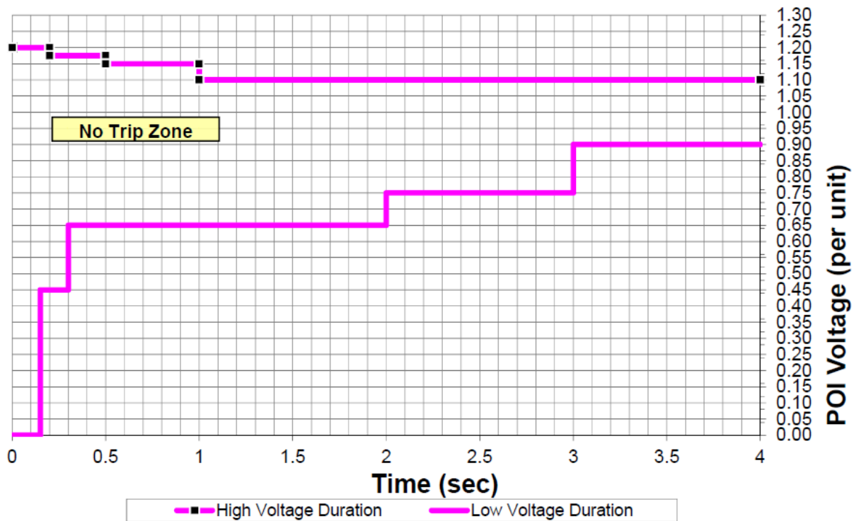
Figure B. Voltage Ride-Through Time Duration Curve, PRC-024 Attachment 2
